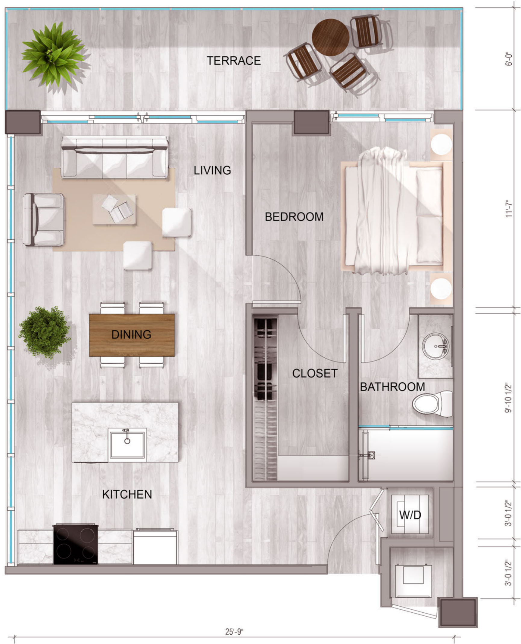
Floor Plan Typical Unit 1-F
